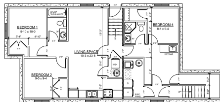
BASEMENT DEVELOPMENT SUITE AREA: 696 SQ.FT
